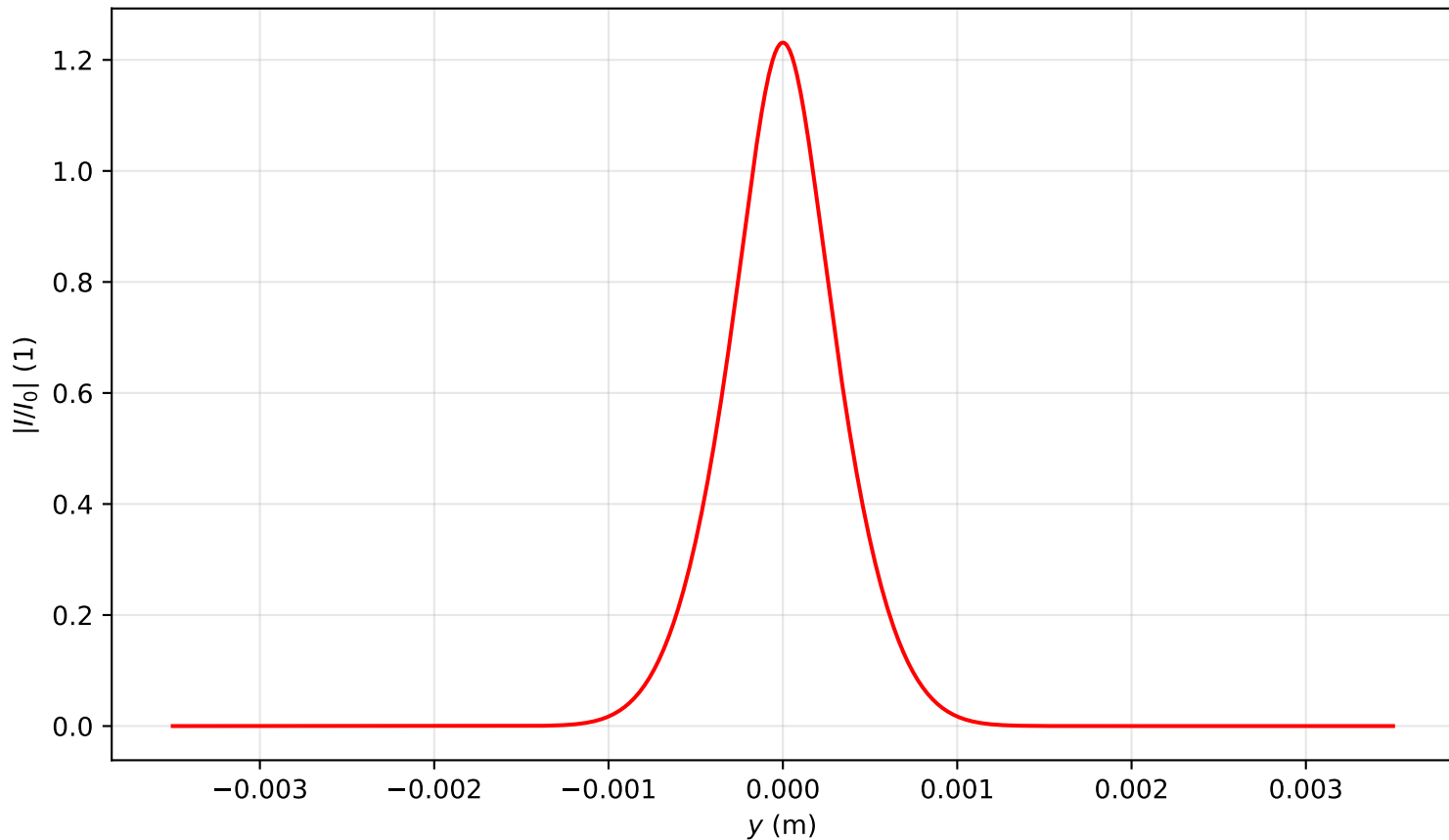
Intensity profile I(x=0, y, z=0.239)/I_0 , P_{in}=3.5P_{cr} , artificial time
